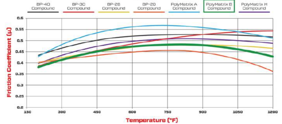
PolyMatrix B Friction Coefficient and Temperature Values
